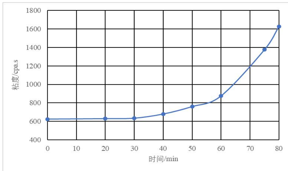
Elapsed time vs viscosity curve at 25℃ (150g)
