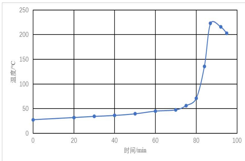
Elapsed time vs Temperature curve at 25℃ (150g)
